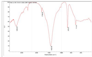
Fig.2 FTIR spectrum of calibration residue
