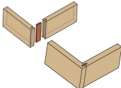
Spline Joint
