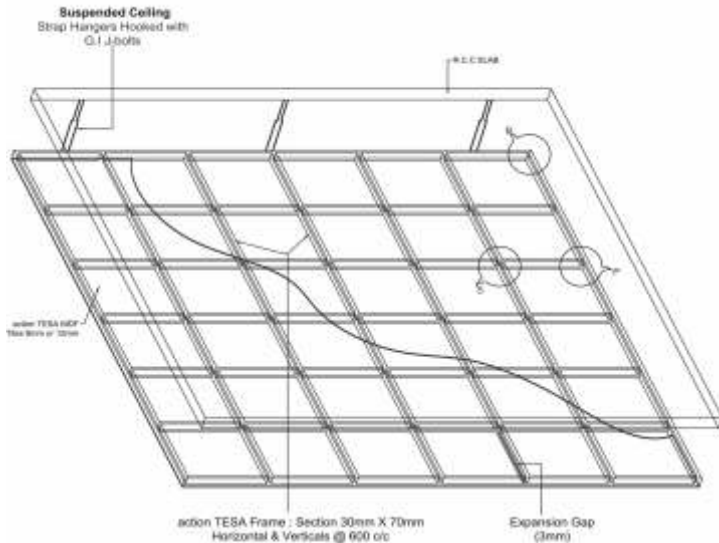
SECTIONAL ELEVATION
